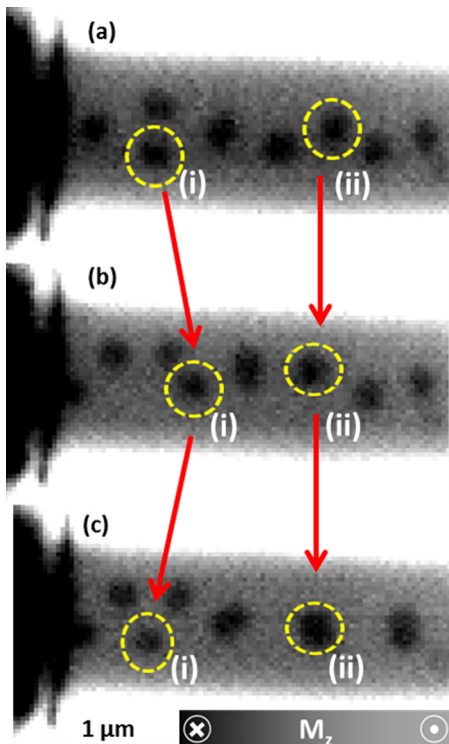
FIG. 4. Room temperature skyrmions nucleated in 1.4 \mu\text{m} \times 5.0 \mu\text{m} micro-wire of [W(5 nm)/CoFeB(0.8 nm)/MgO(2 nm)] 10 /Ta(5 nm) (a). Subsequently nucleated skyrmions are moved forwards and backwards by applying current pulses with opposite polarity (b) and (c). Highlighted skyrmion (i) is moved forward (current applied along the wire from left to right) and backward (reversed polarity). Skyrmion (ii) is an example of a pinned skyrmion that does not move at this current density.
